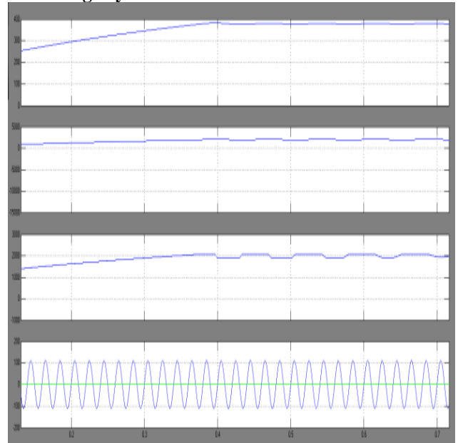
Fig 13. Transition process between ModelI and ModelIII.
