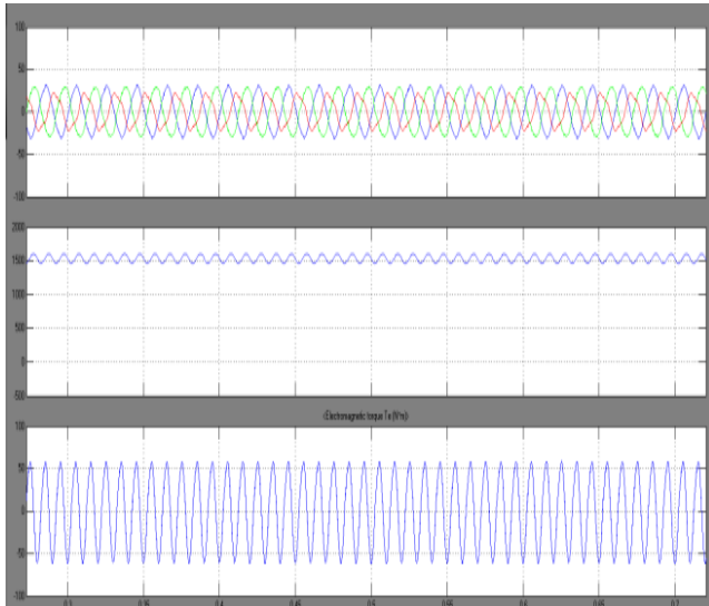
Fig 16. simulation wave form of DC microgrid with Induction Motor stator current, speed and electromagnetic torque.
