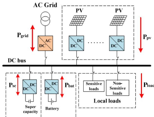
Fig 1. DC microgrid with hybrid storage system.
