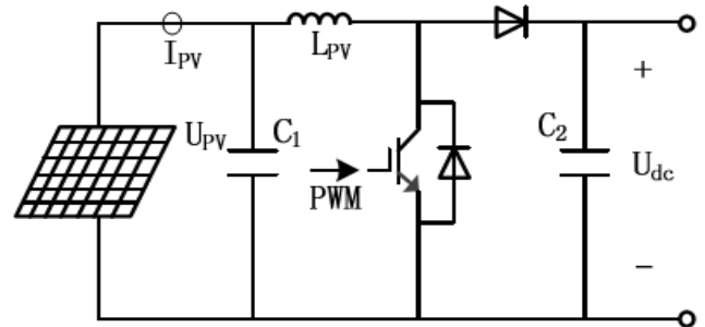
Fig2. DC/DC converter of PV module with MPPT function.
