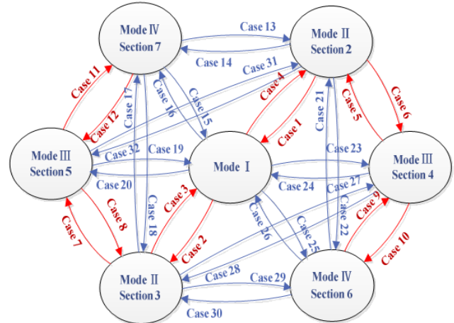
Fig 6. Mode transition mechanism.
