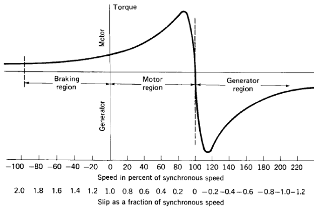
Fig 10. AC Induction Motor Speed-Torque Characteristic.
