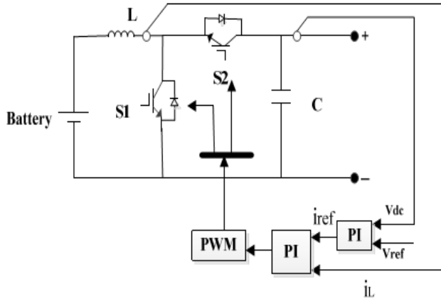
Fig 4. Control strategy of the bi-directional DC/DC converter.
