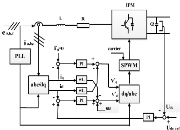
Fig 5. Control strategy of the bi-directional DC/AC converter.
