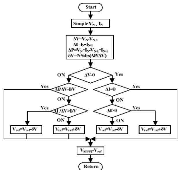
Fig3. Flowchart of the variable step size INC MPPT algorithm
