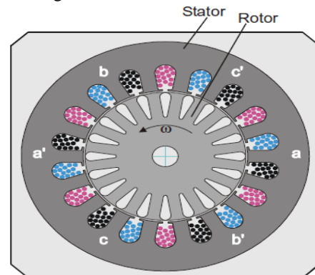
Fig 9. 3-Phase AC Induction Motor.
