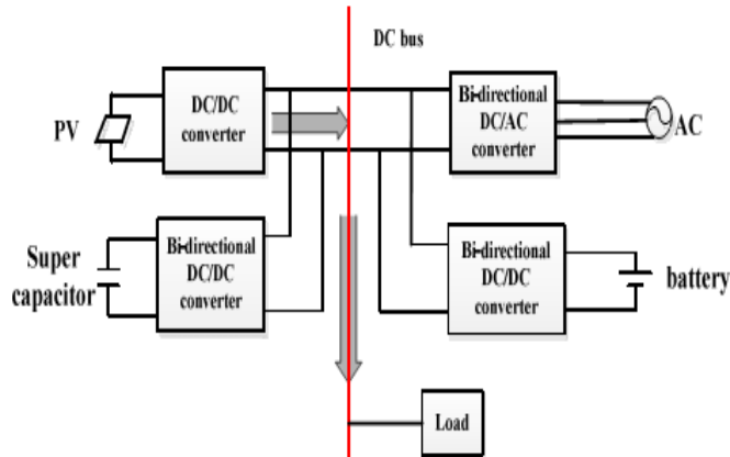
Fig 8. Power flow of modelI.
