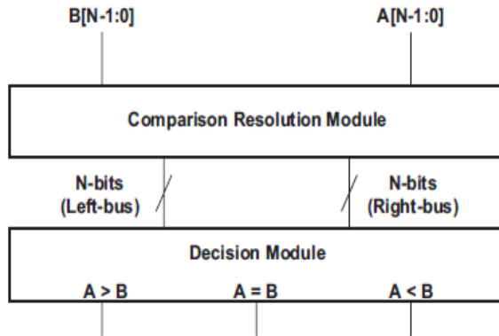
Fig.1. Block diagram of our comparator architecture, consisting of a comparison resolution module connected to a decision module.
