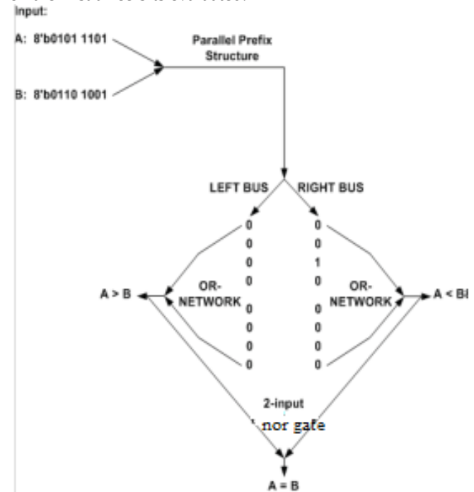
Fig. 2. Example 8-b comparison.
