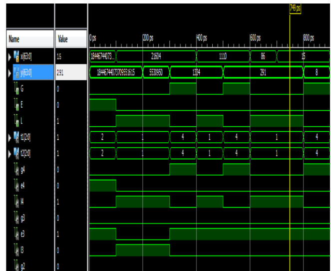
Fig7. Simulation Result.
