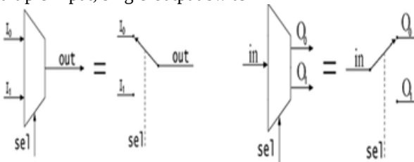
Fig5. Switch.
