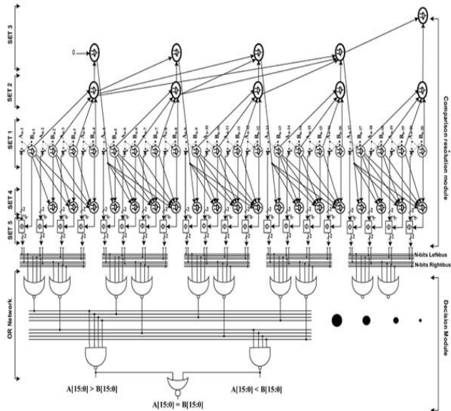
Fig4. Implementation details for the comparison resolution module (sets 1 through 5) and the decision module.
