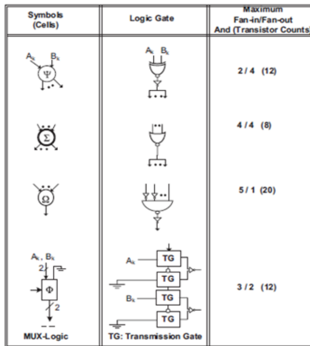
Fig.3: Logic Gate Representations For Symbols.
