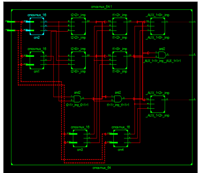
Fig6. Internal Schematic For Comparator For 64 Bit.
